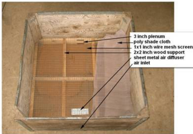
Figure 7. Top view of a grain drying bin, showing poly shade cloth (partly removed), 1 x 1 inch wire mesh screen, 2 x 2 inch wood support for wire screen and sheet metal air diffuser.
